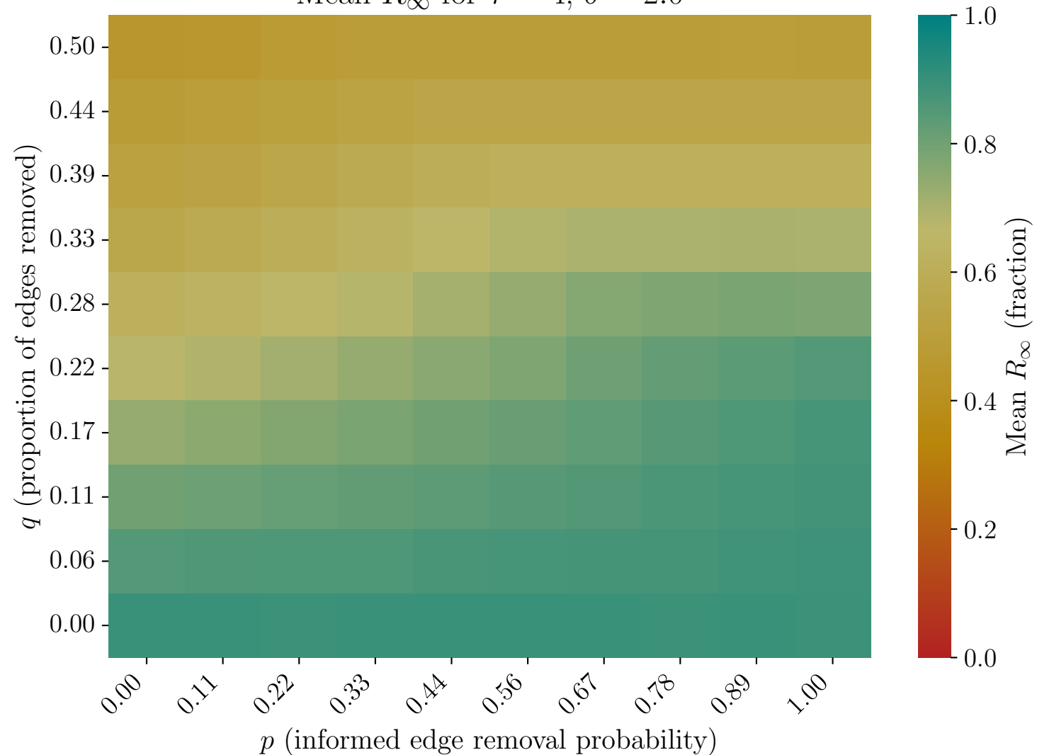
Mean R_\infty for \tau = 4 , \delta = 2.0
