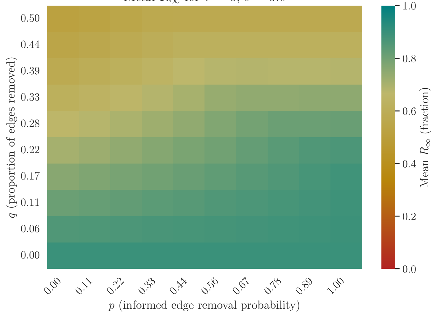
Mean R_\infty for \tau = 5 , \delta = 3.0
