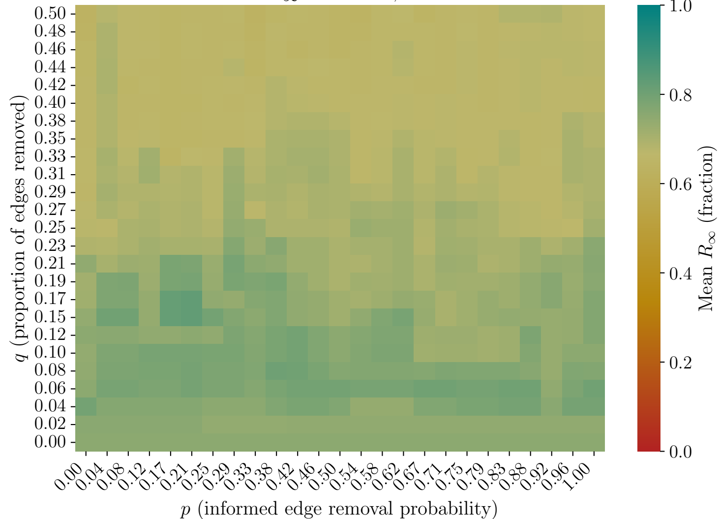
Mean R_\infty for \tau = 9 , \delta = 1.0
