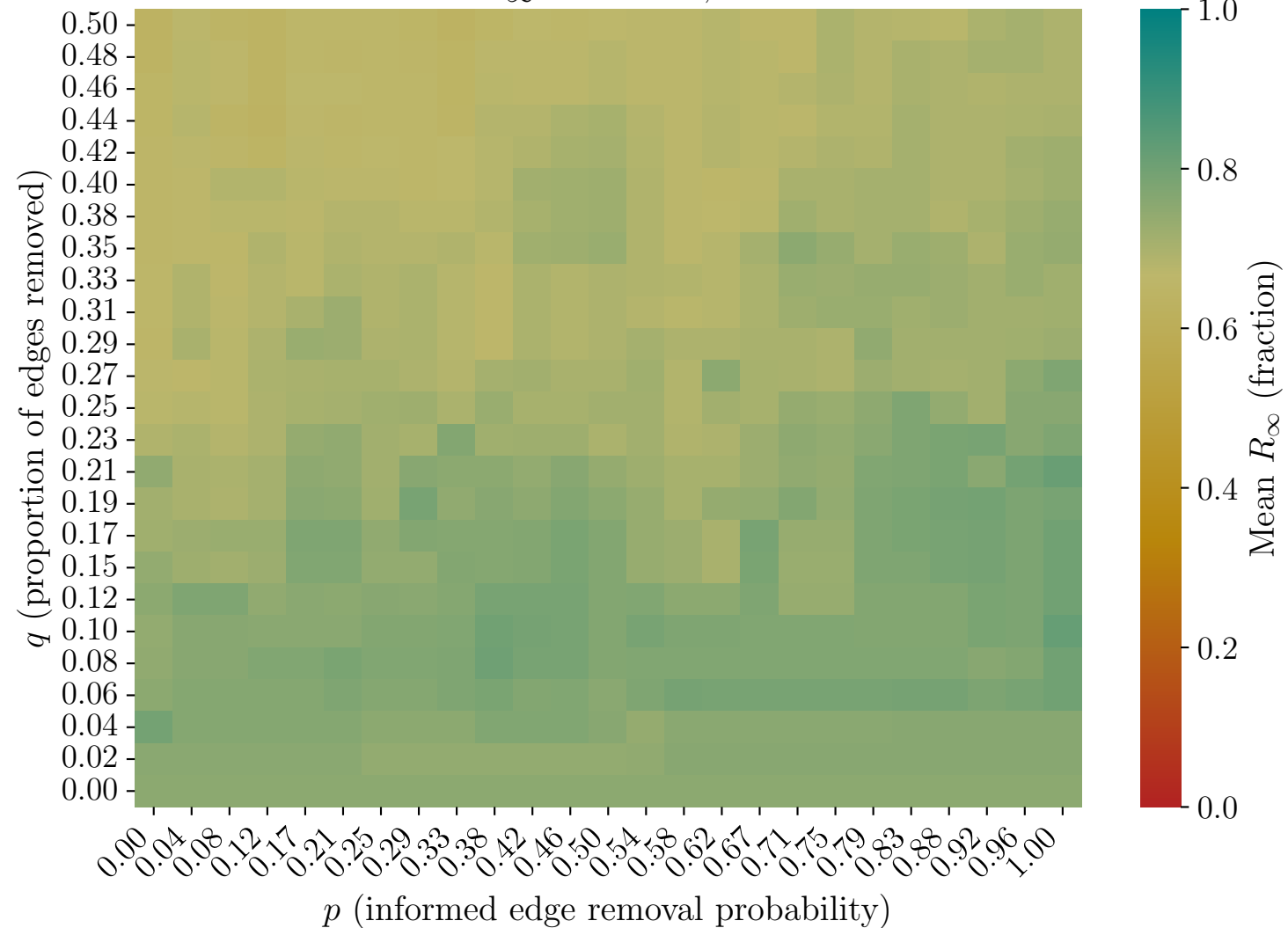
Mean R_\infty for \tau = 9 , \delta = 2.0
