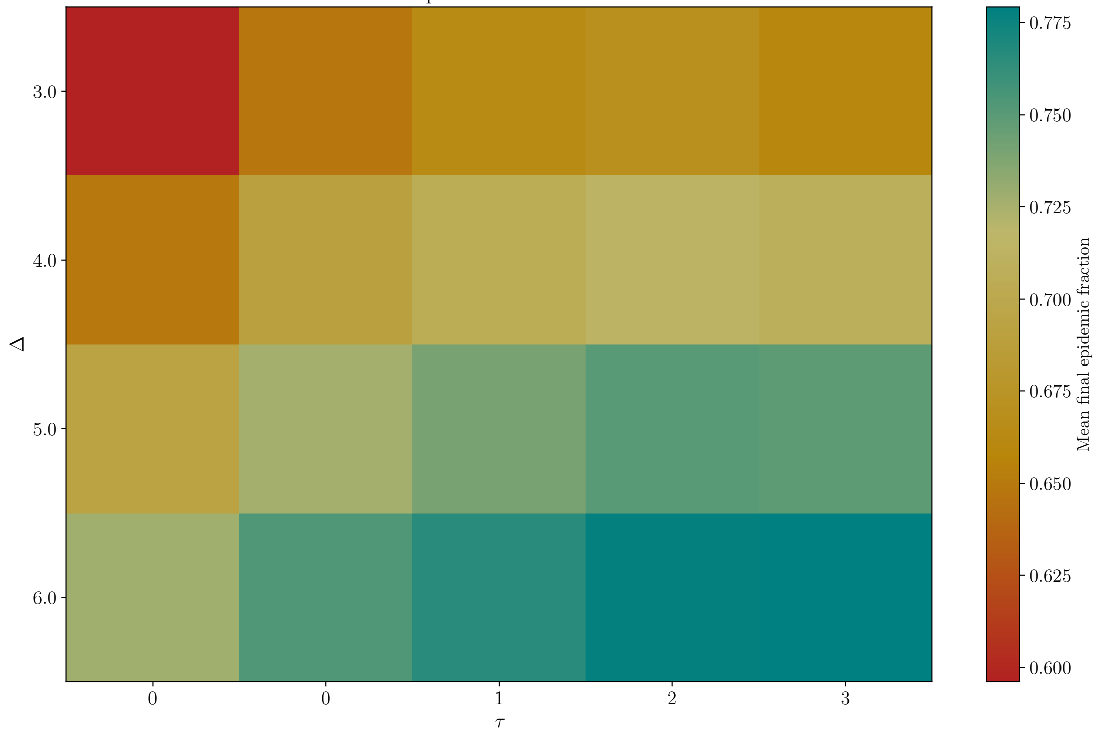
Mean Final Epidemic Fraction vs \tau and \Delta
