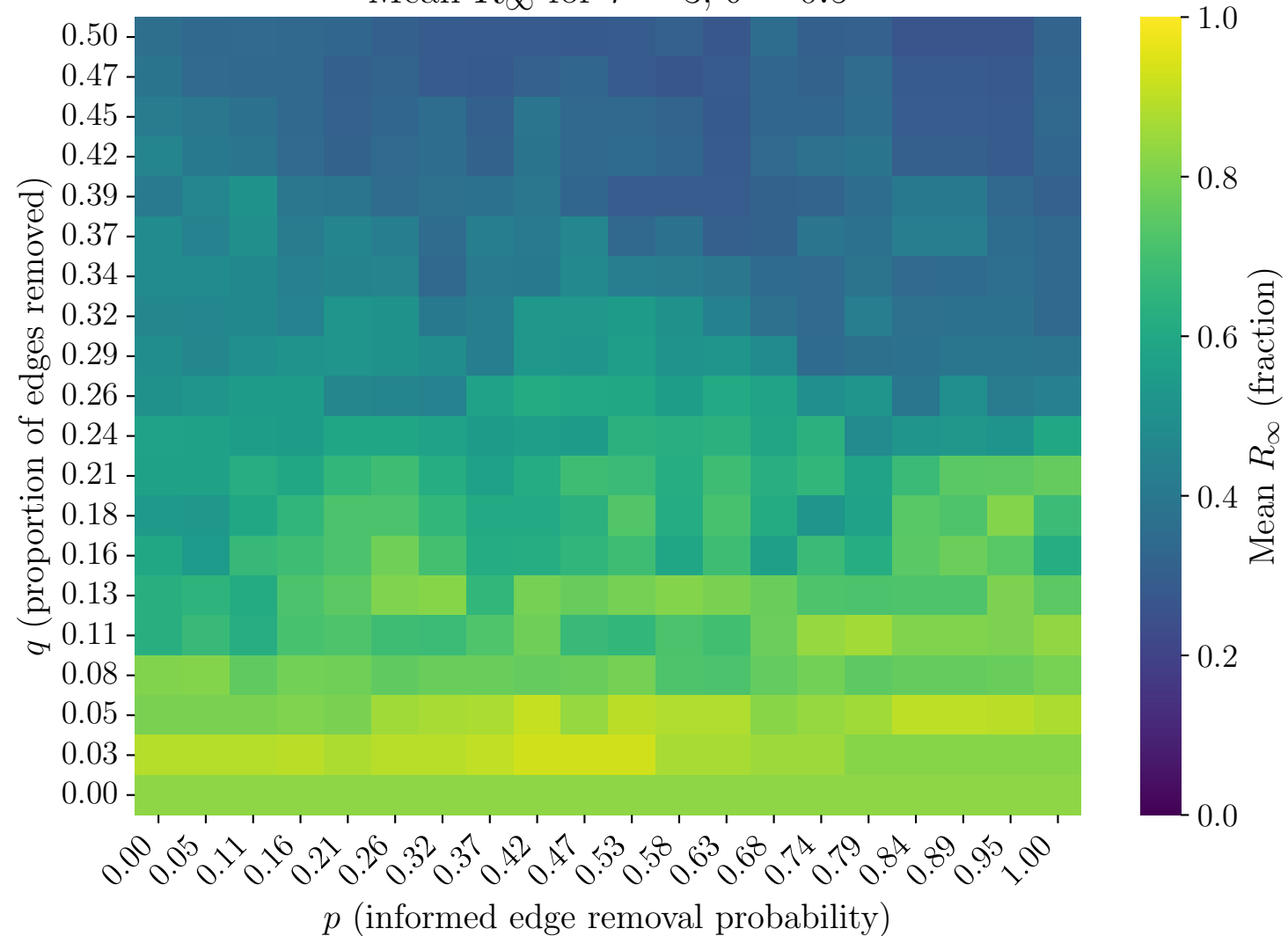
Mean R_\infty for \tau = 3 , \delta = 0.5
