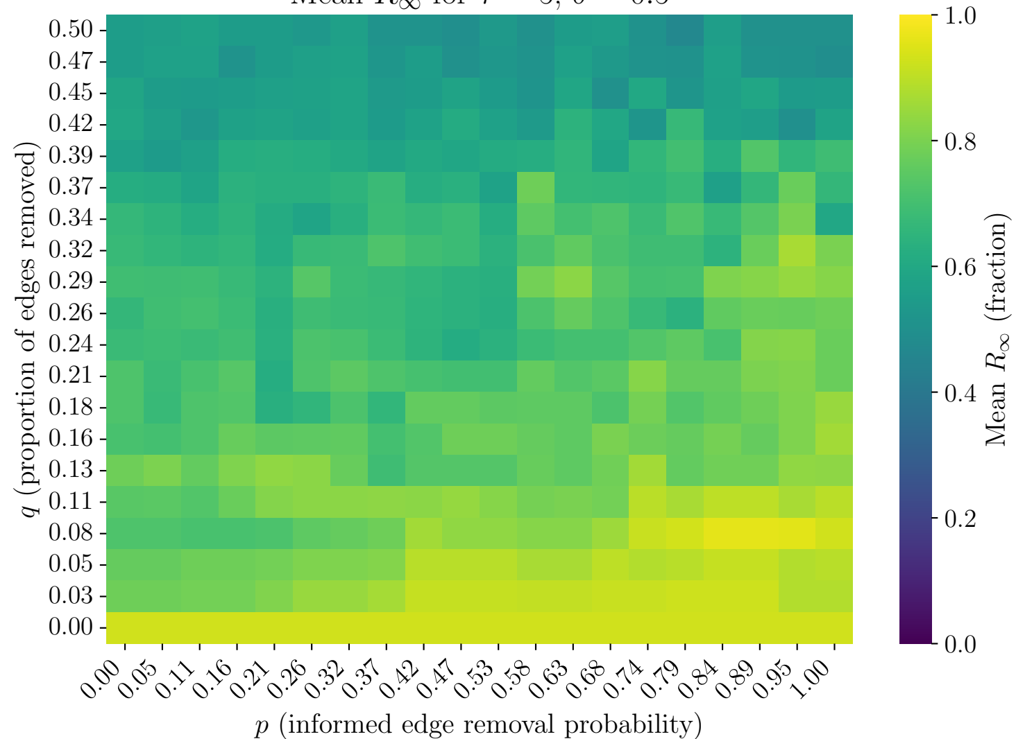
Mean R_\infty for \tau = 5 , \delta = 0.5
