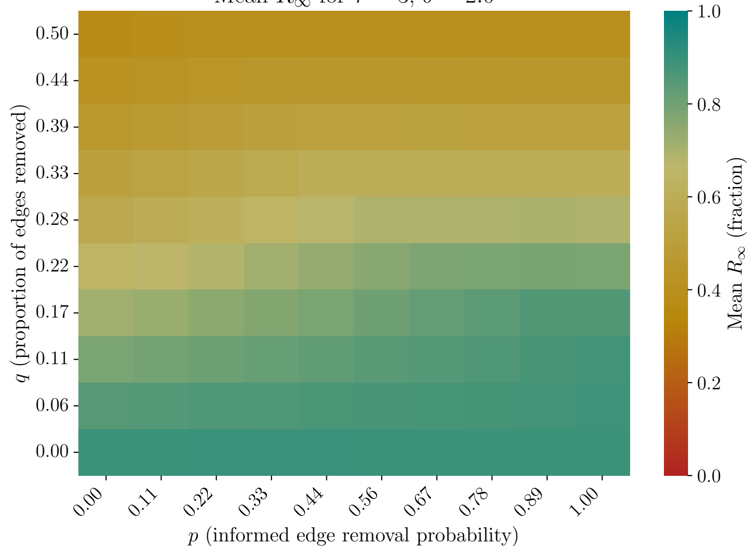
Mean R_\infty for \tau = 3 , \delta = 2.0
