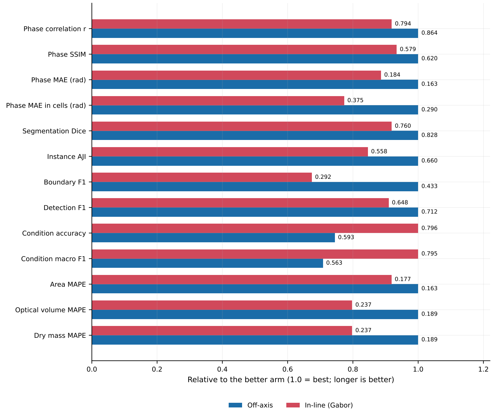
Off-axis versus in-line Gabor, all reported axes annotations are the raw values
