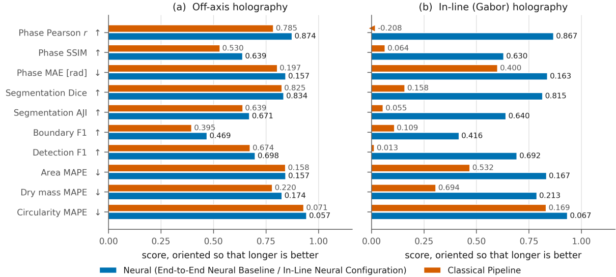
Figure 2: Neural and tested classical pipelines, oriented so that longer bars are better (error metrics drawn as 1 - \text{error} , raw value printed). (a) Off-axis, 113 test fields; End-to-End Neural Baseline, mean over three seeds. (b) In-line, the 107 correctly paired test fields; In-Line Neural Configuration, one run. The negative phase correlation of the classical in-line reconstruction is drawn at zero with a left-pointing marker.
