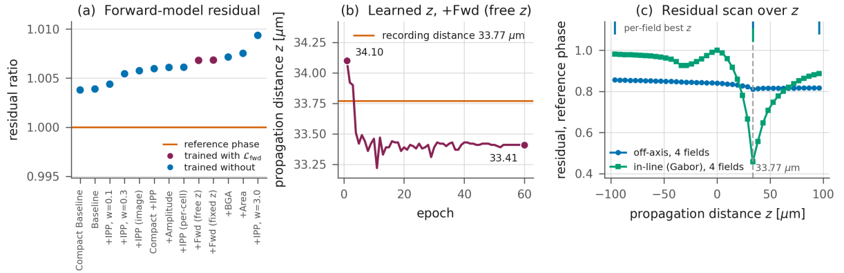
Figure 7: Forward-model consistency. (a) Residual of each trained off-axis configuration on the 113 test fields divided by the residual obtained with the reference phase (three-seed means for the baseline and the two +IPP configurations, single runs otherwise). (b) Propagation distance of +Fwd (free z ) per epoch, initialised at the recording distance. (c) Residual computed from the reference phase as a function of z on four validation fields per geometry ( 4.81 \mu\text{m} grid); ticks at the top mark each field’s best distance, and the dashed line the recording distance.
