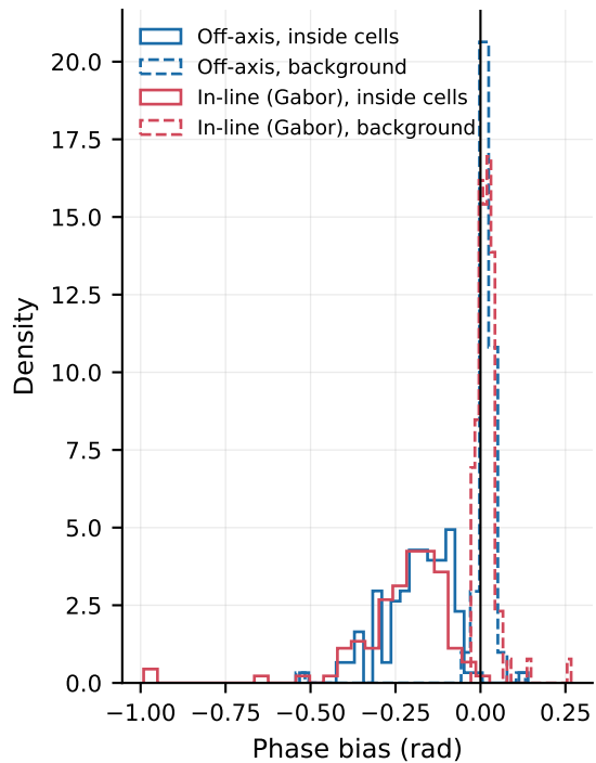
Where the phase error sits mass integrates only the inside
