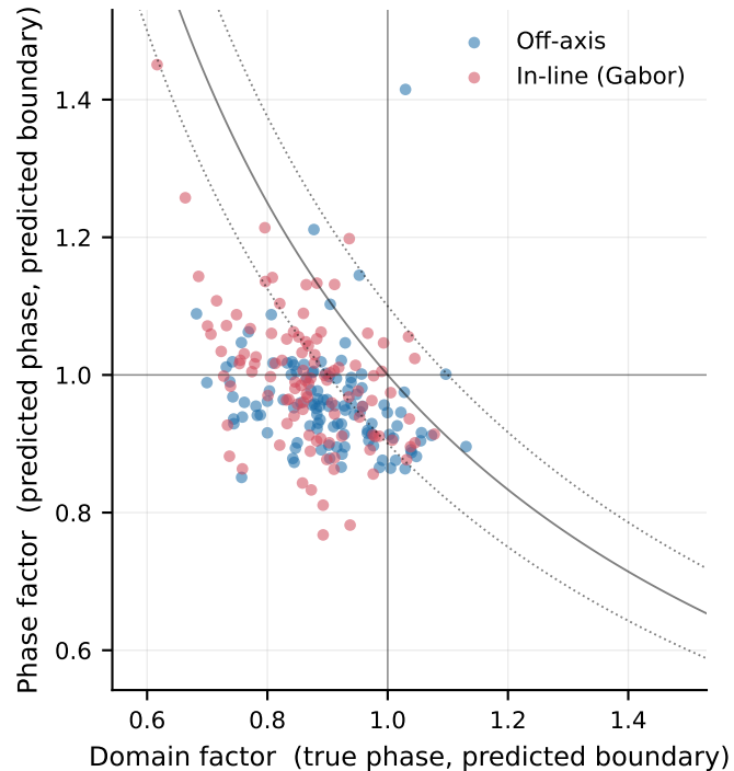
Mass ratio factorised solid line = correct mass
