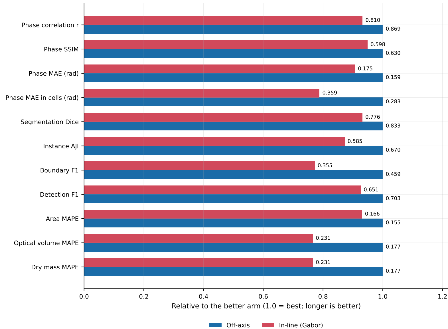
Off-axis versus in-line Gabor, all reported axes annotations are the raw values
