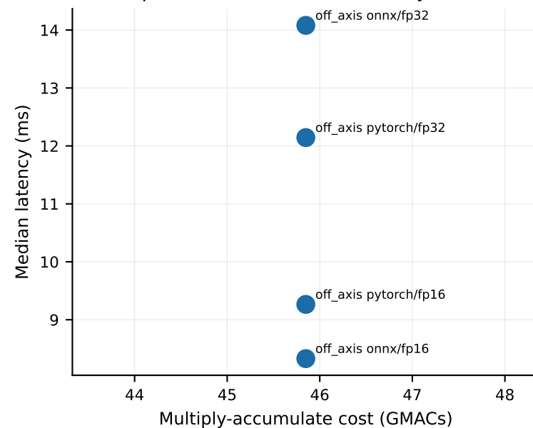
Compute cost against measured latency departure from a line = memory bound
