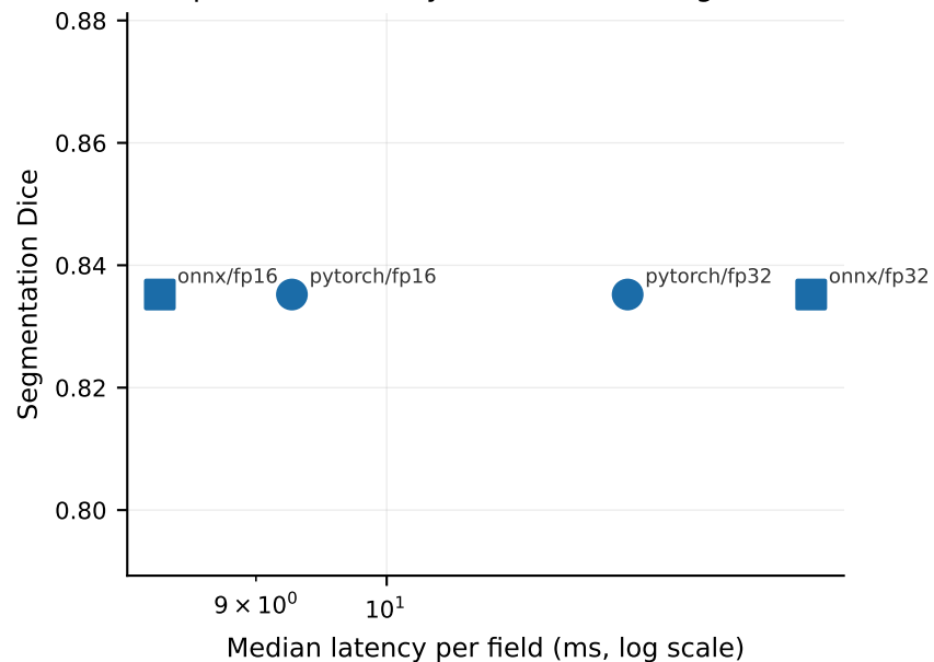
Accuracy against inference cost
