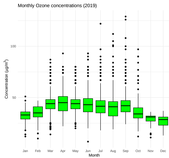
Figure 2: 2019 monthly Ozone levels
