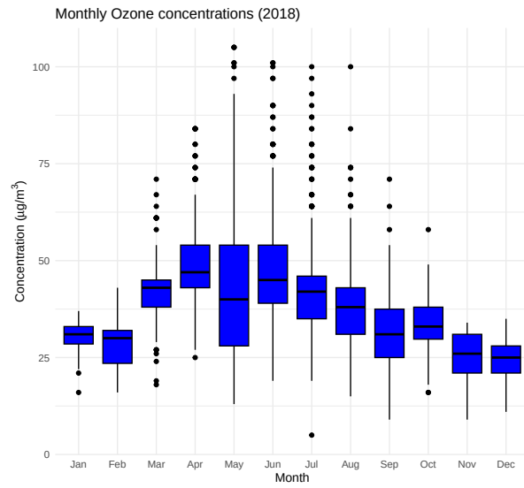
Figure 1: 2018 monthly Ozone levels
