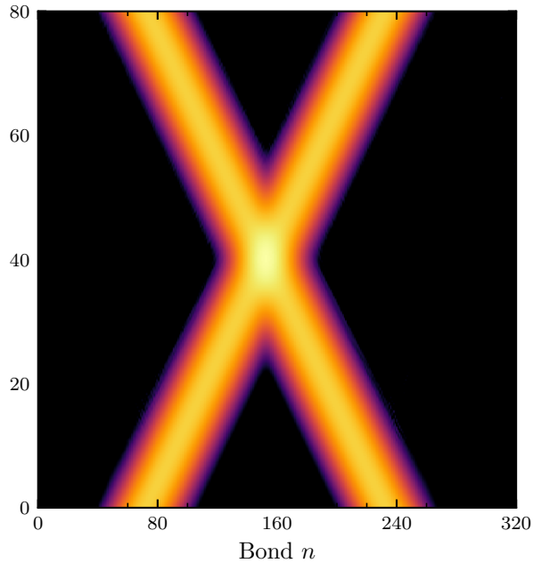
(a) Integrable h_x = 1.06, \quad h_z = 0
