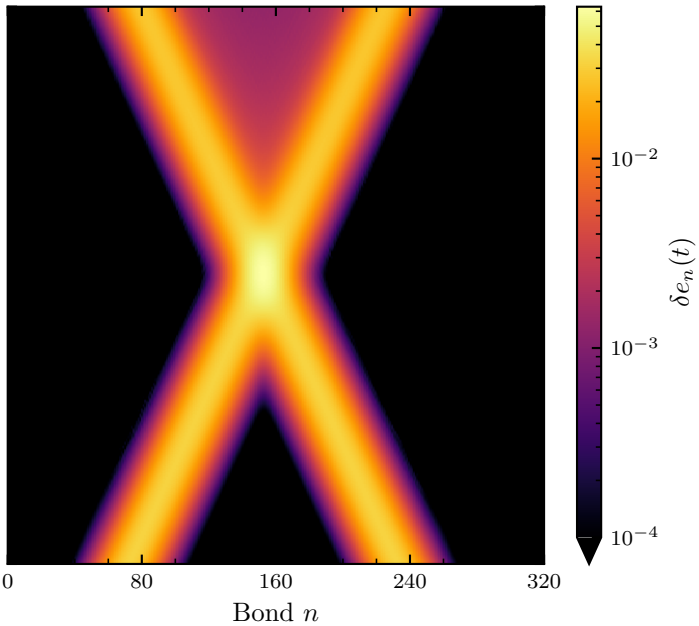
(b) Non-integrable h_x = 1.06, \quad h_z = 0.006
