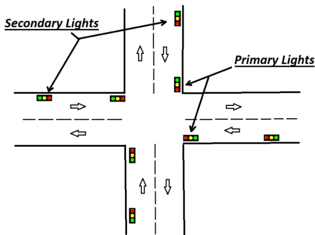
Fig 4: Concept of Primary & Secondary Lights
