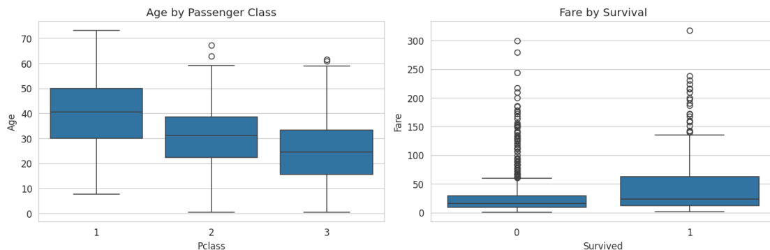
Figure 4: Age varies by passenger class; Fare shows a wider, higher spread among survivors.
