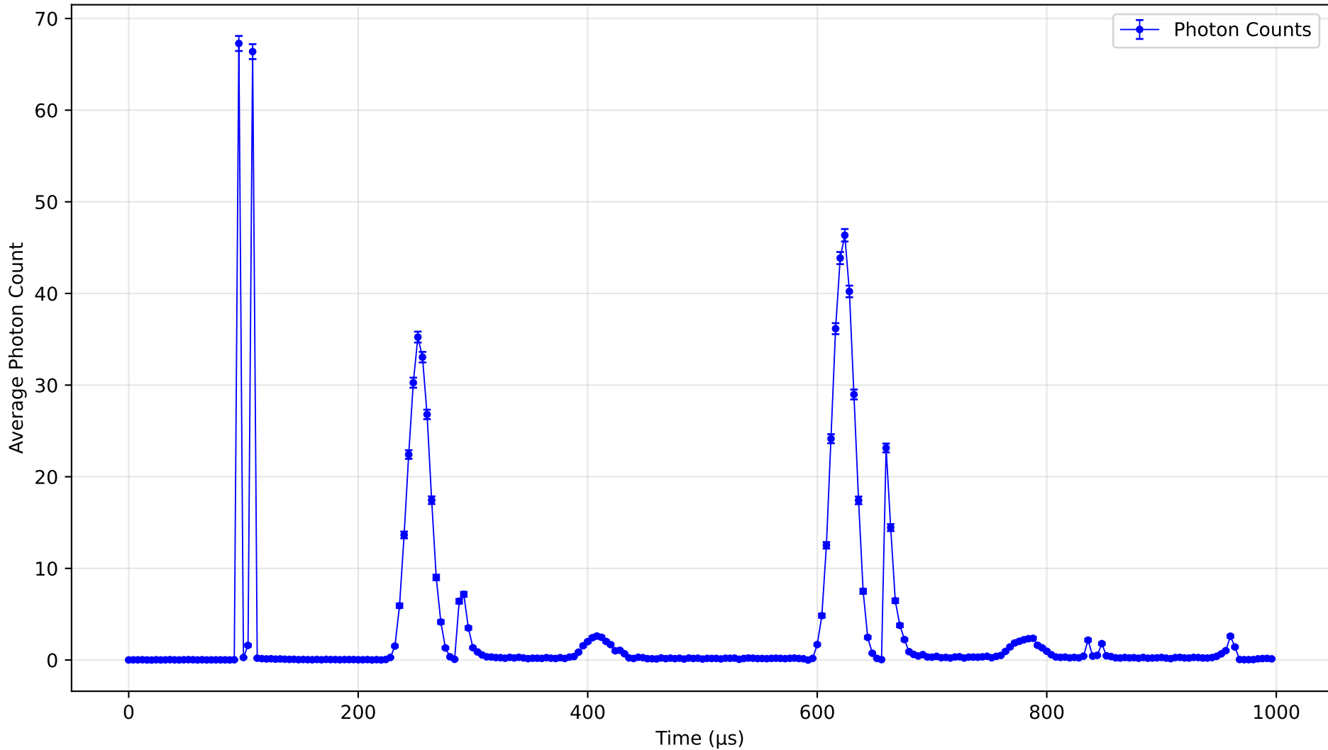
Photon Counts vs Time (Detuning 0)
