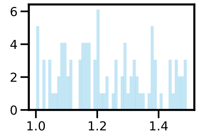
q_i [GB]
