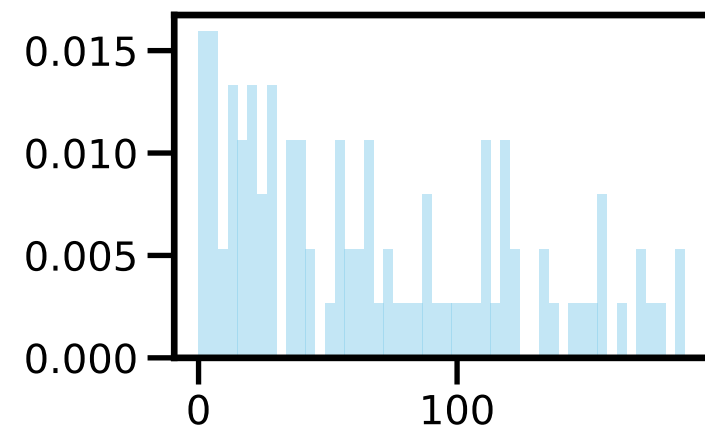
q_e [GB]
