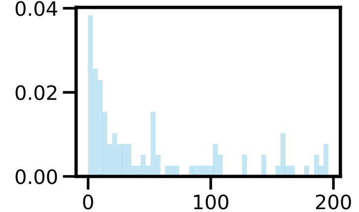
q_i [GB]
