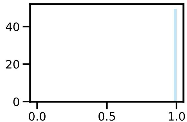
stable
