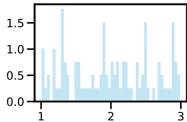
stable
