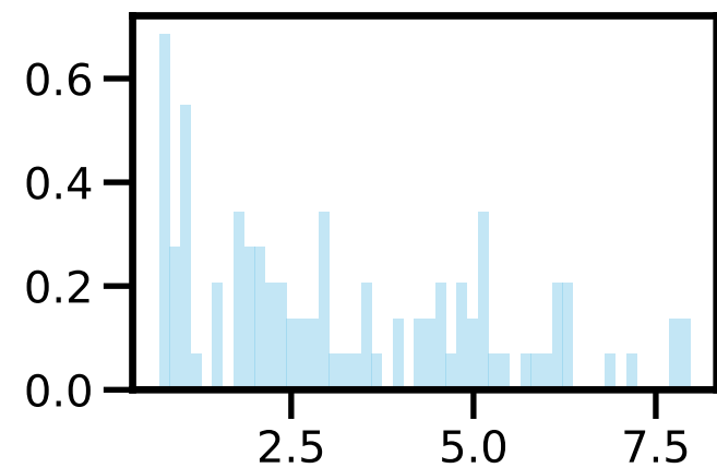
Z_{eff}
