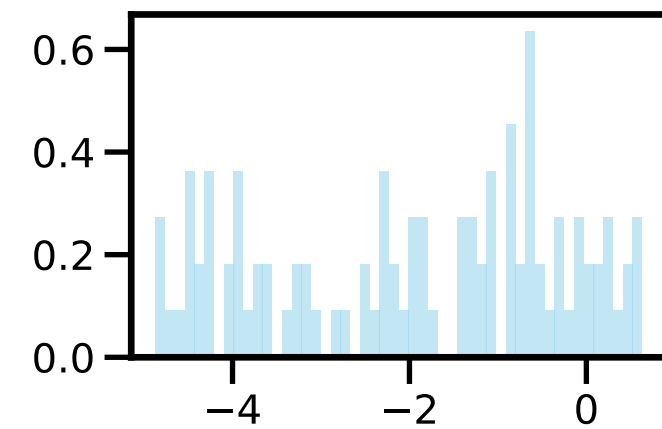
q_e [GB]
