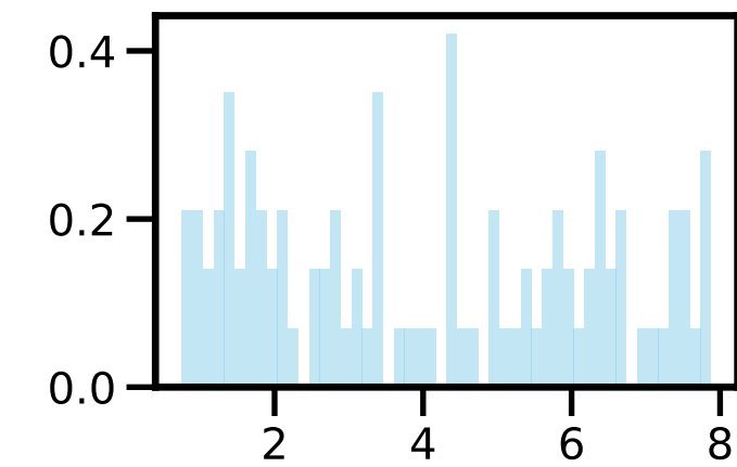
Z_{eff}
