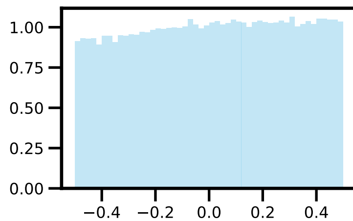
q_i [GB]
