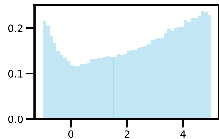
Z_{eff}
