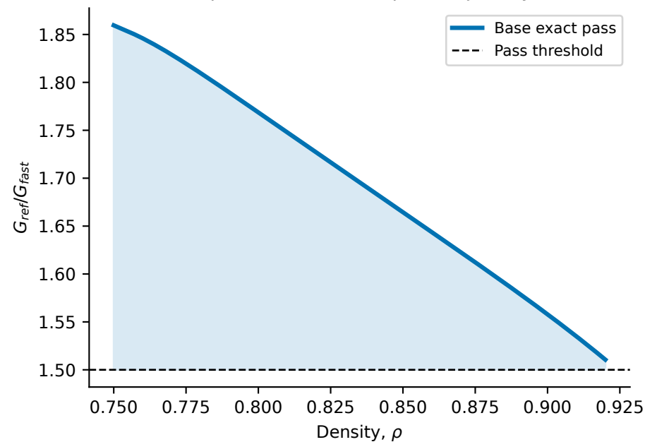
Ablation attribution
