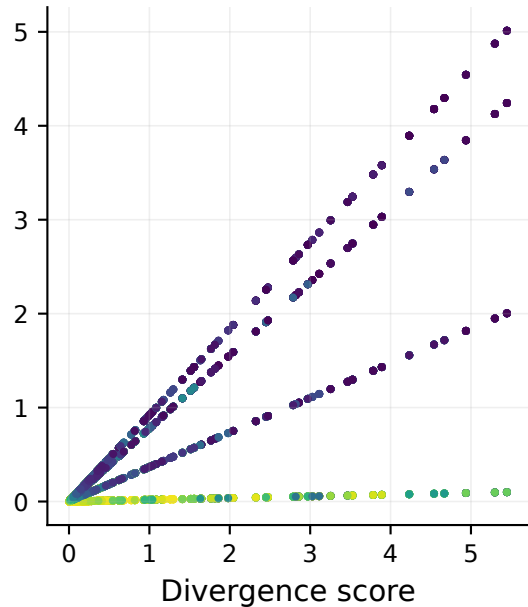
Persistence score
