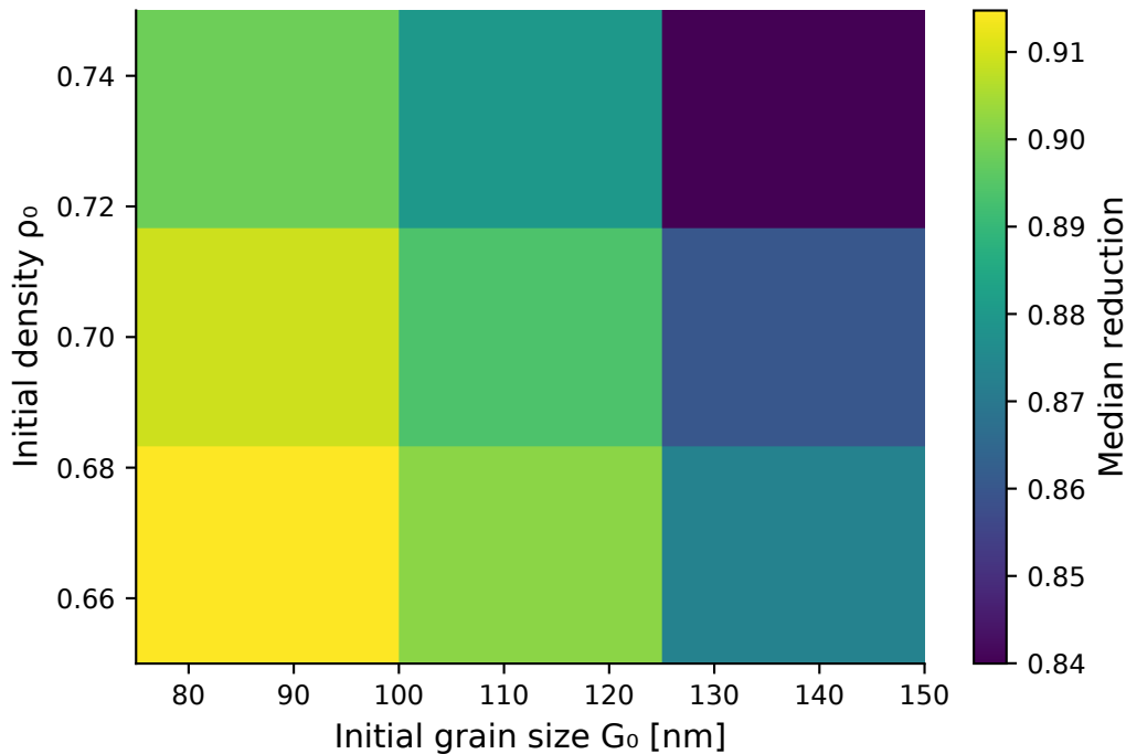
Candidate 693168: robustness
