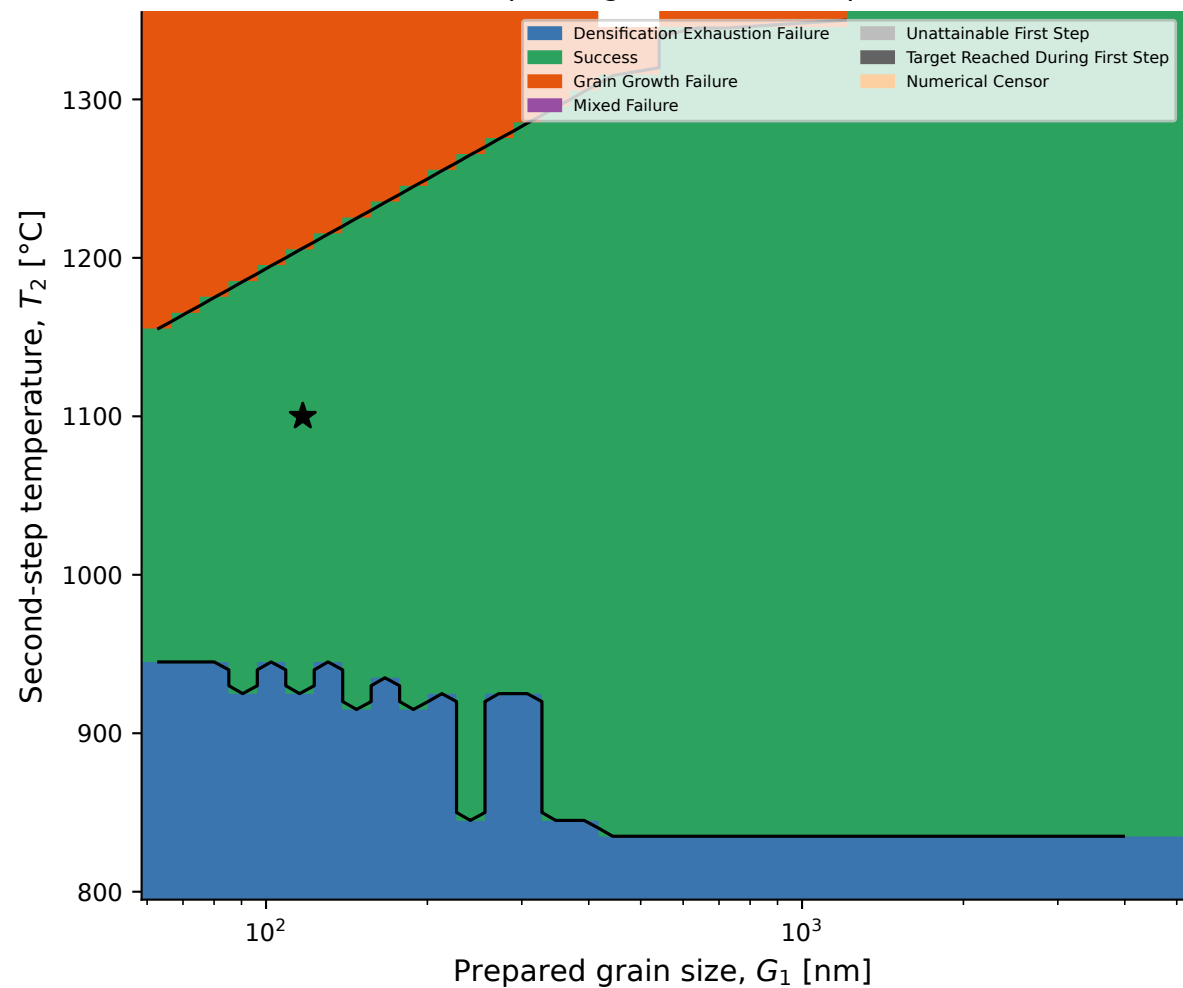
Prepared grain size- T_2 map
