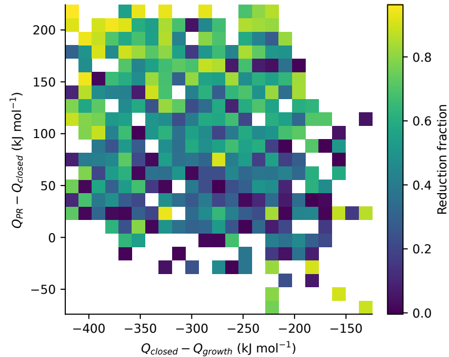
Exact high-density reduction
