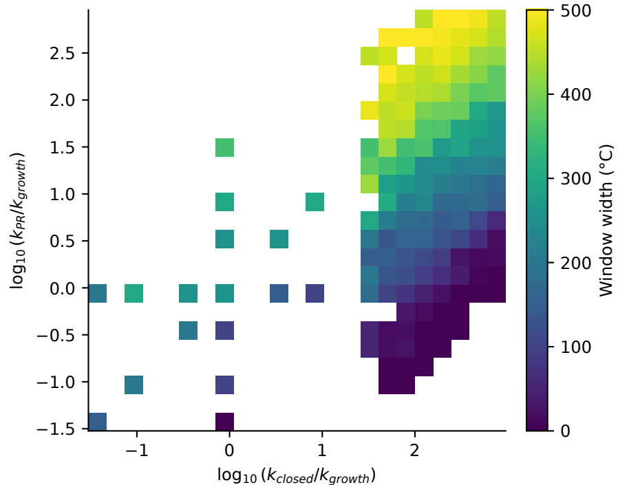
Exact Chen-window width
