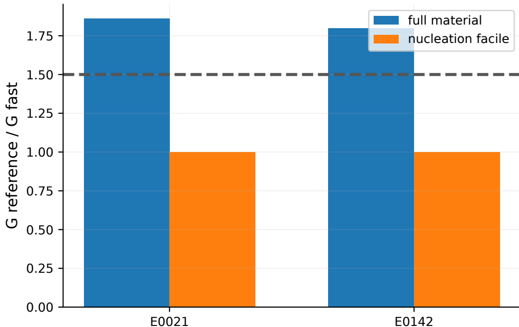
Frozen fast-firing envelope
