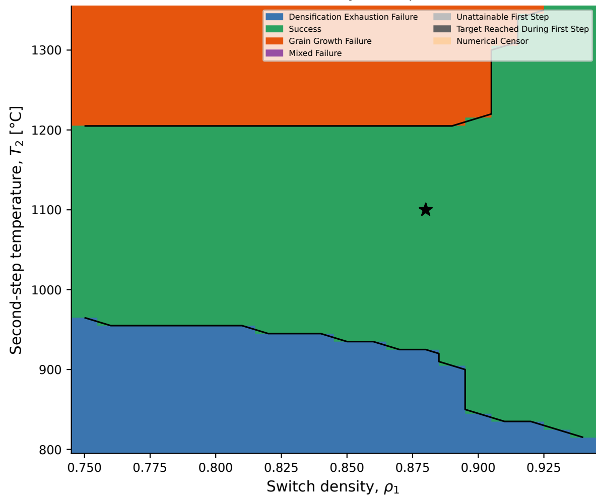
Switch-density- T_2 map
