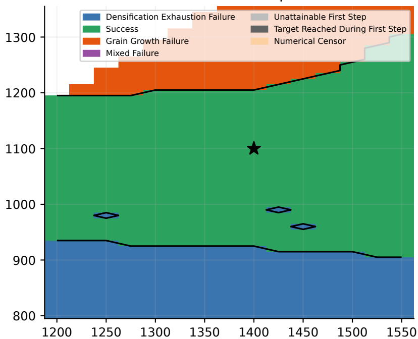
Filled Chen map
