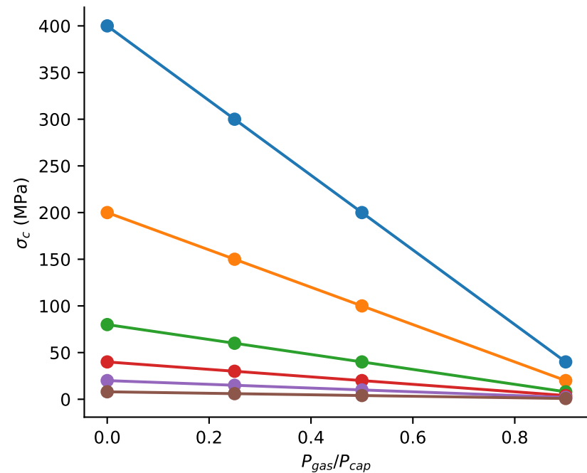
Gas counterpressure and pore-radius limits
