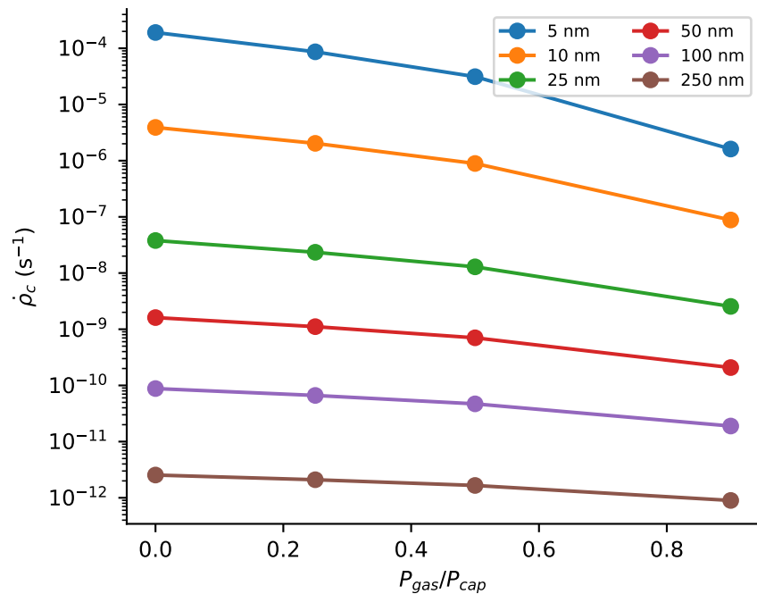
Gas counterpressure and pore-radius limits
