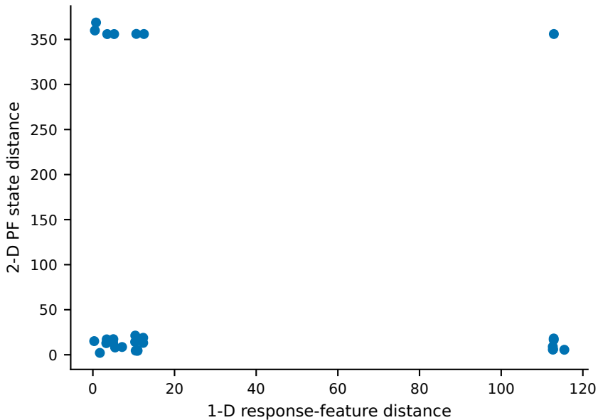
Poor 1-D to 2-D distance transfer
