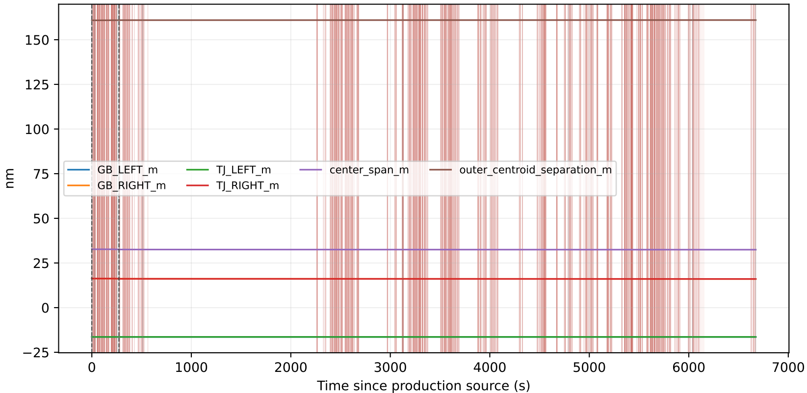
Axial geometry
