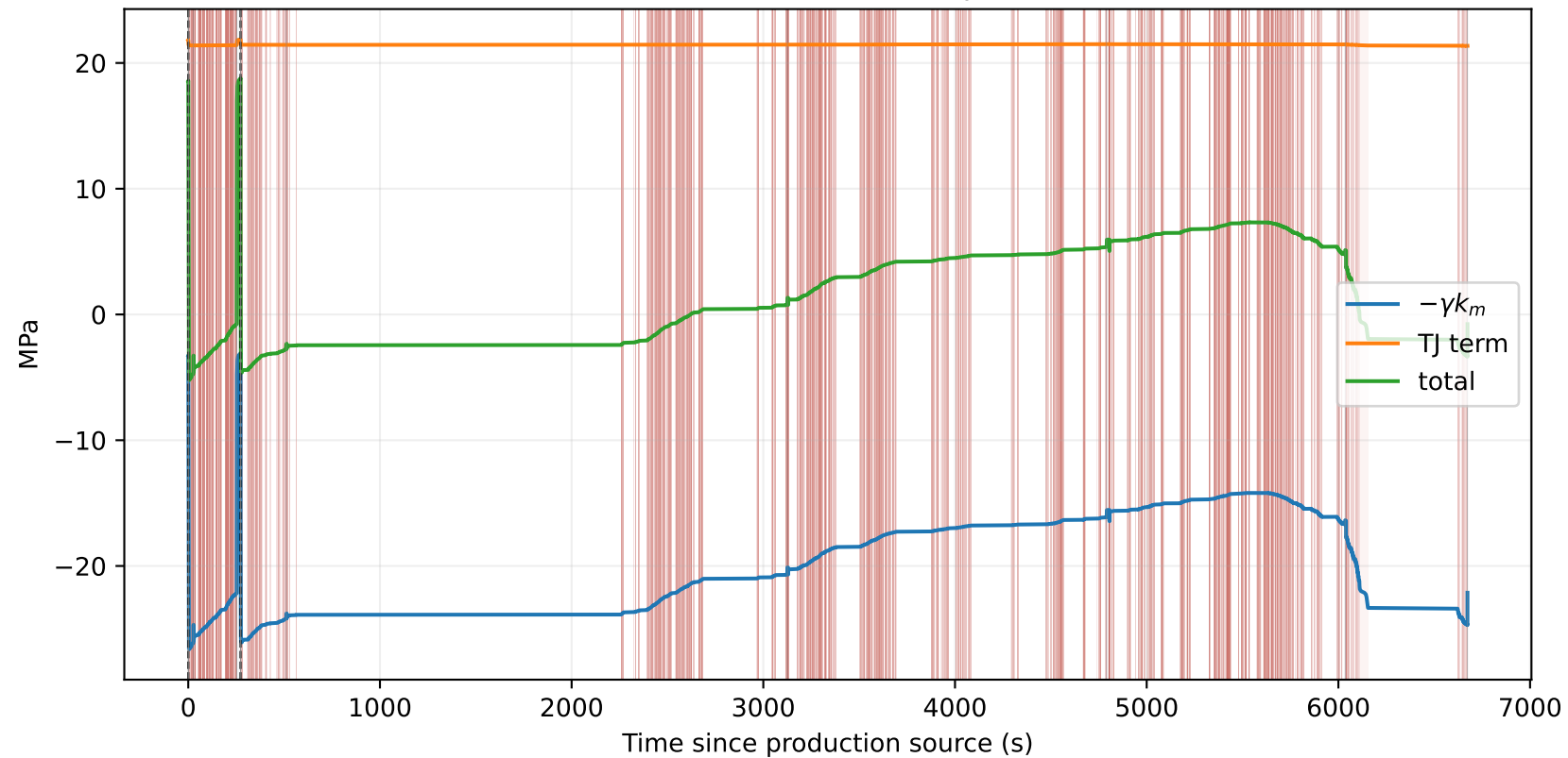
LEFT center stress decomposition
