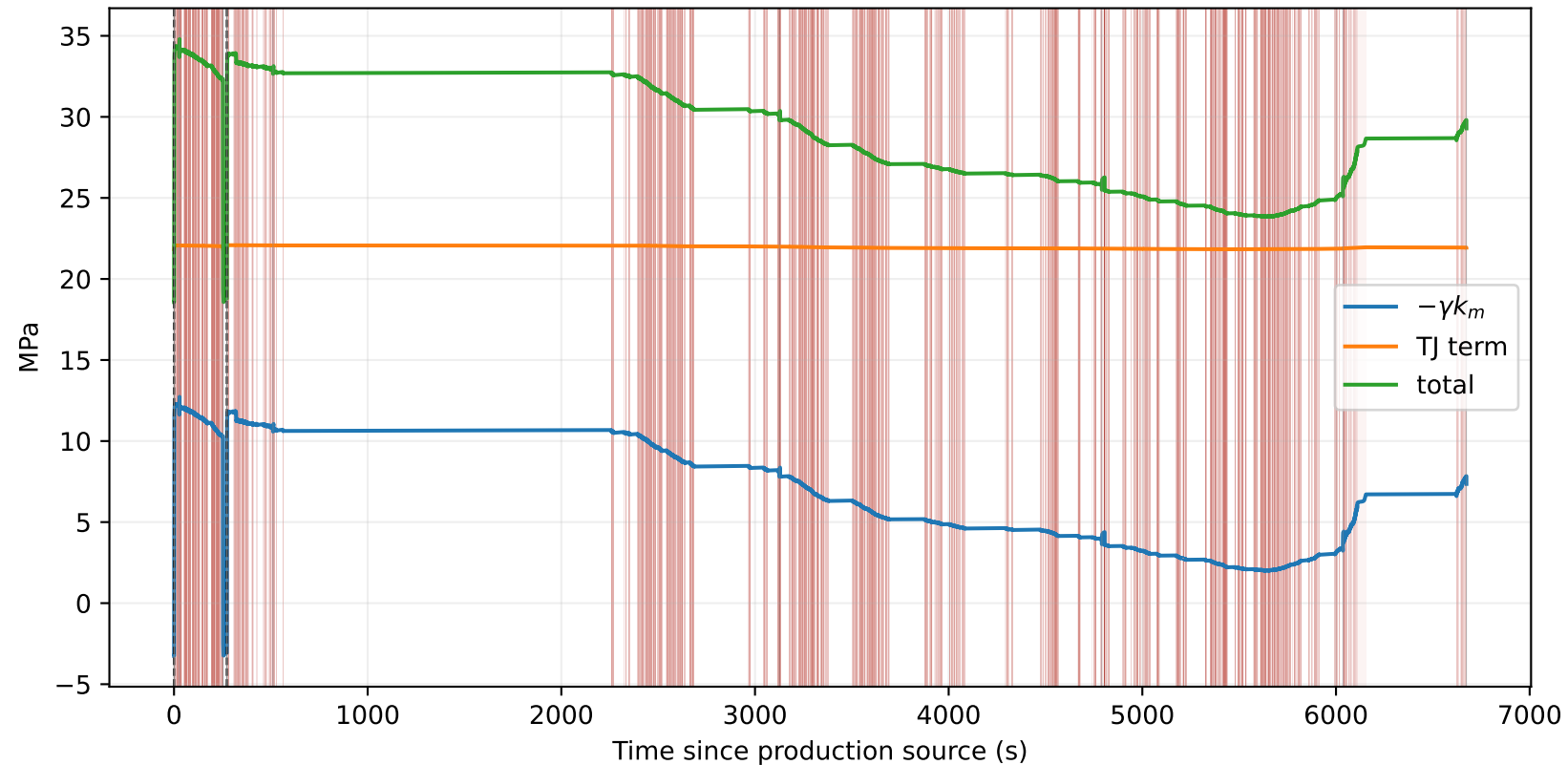
RIGHT center stress decomposition
