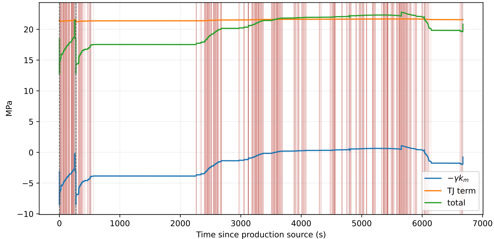
RIGHT outer stress decomposition
