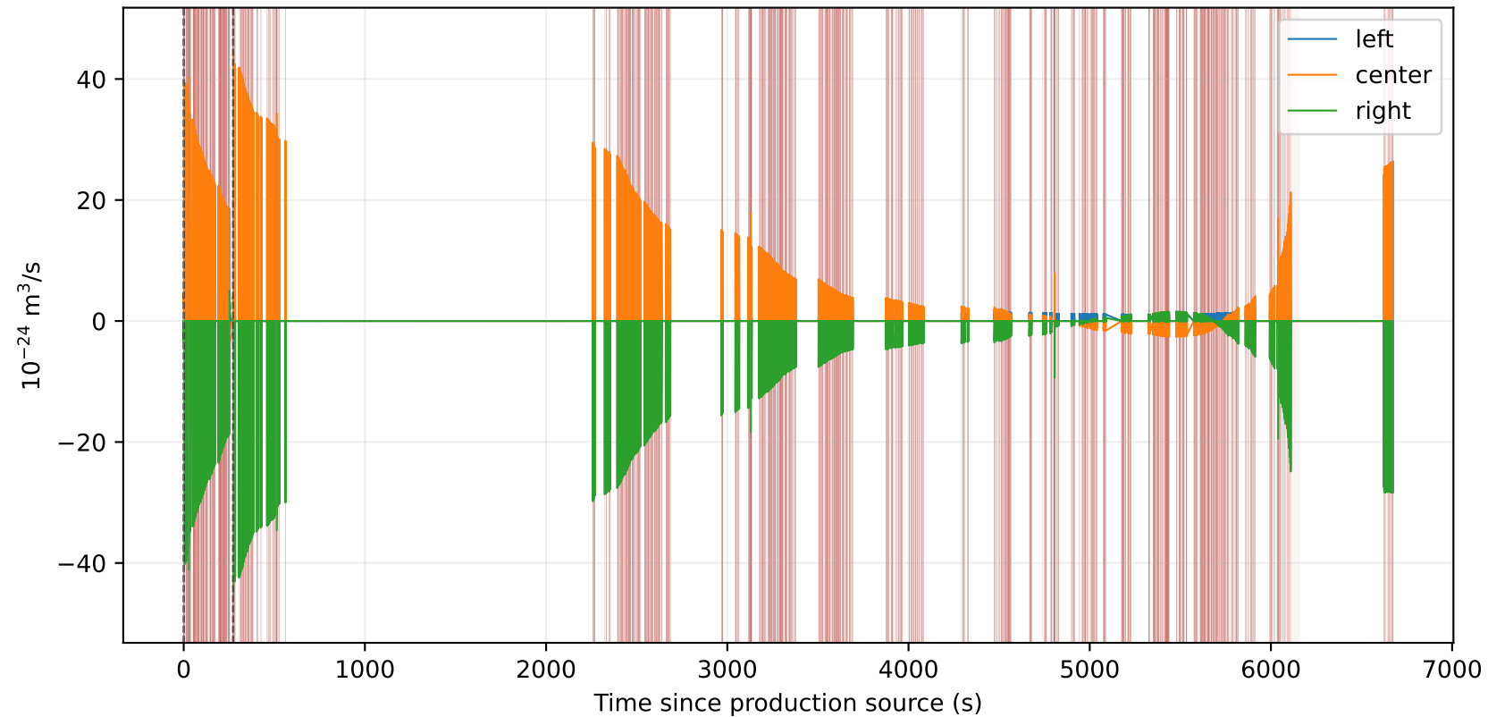
Phase-wise grain volume rate
