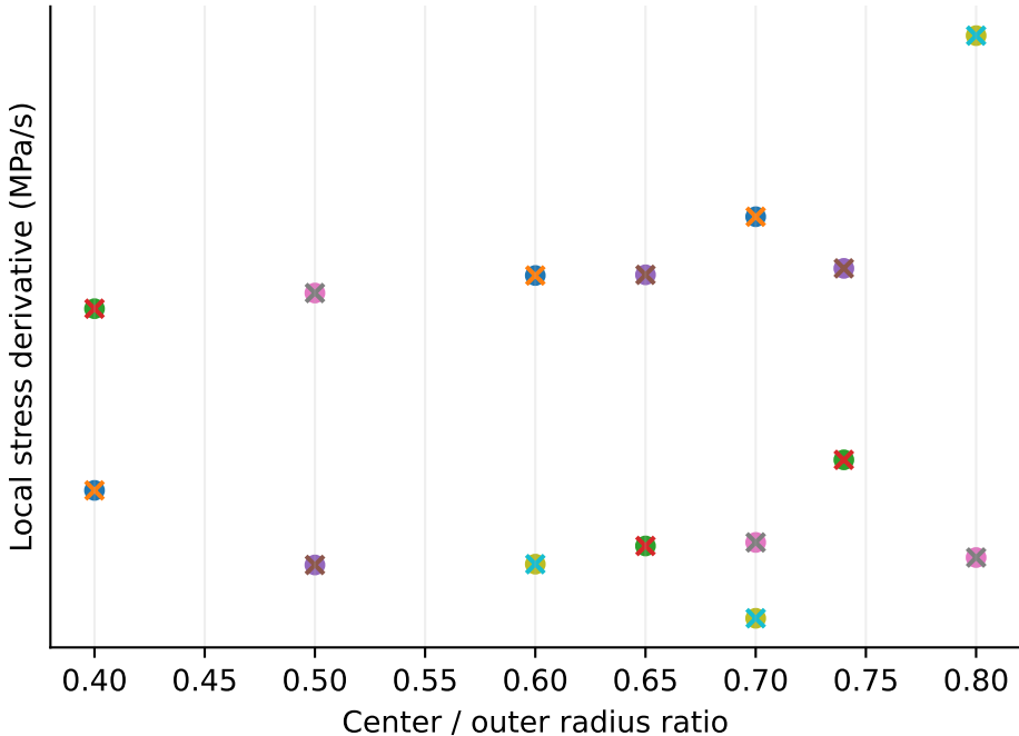
1000 native steps immediately after cleanup Early relaxation slopes must not be extrapolated to a root event
