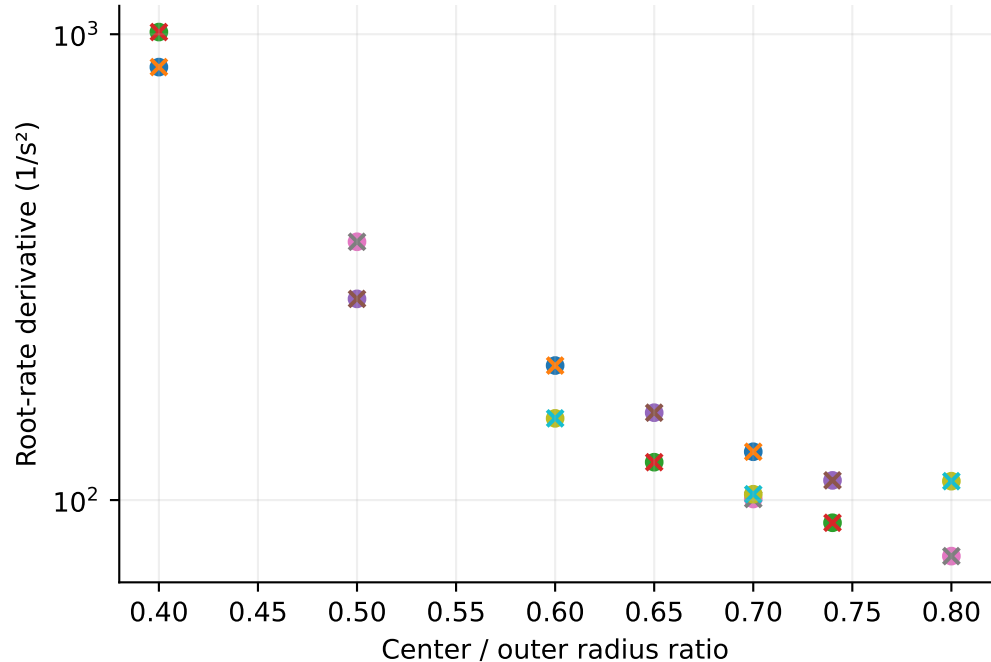
1000 native steps immediately after cleanup Early relaxation slopes must not be extrapolated to a root event
