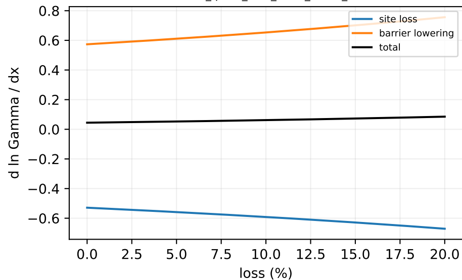
C4: Ro100_q0.75_L12W_r1.40_th140_km+5
