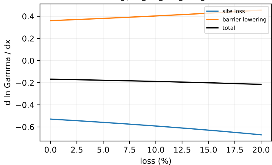
C3: Ro150_q0.65_L12W_r1.60_th170_km-10
