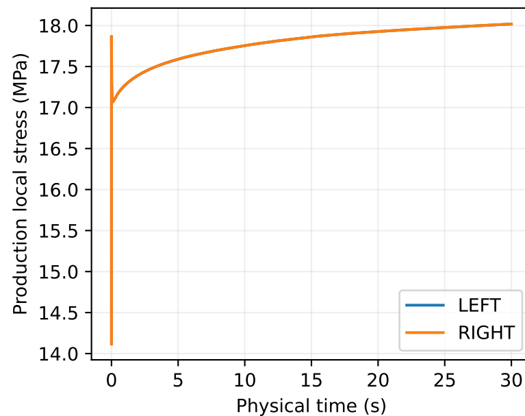
Selected 0.65 events-off reload — unchanged kinetics and 1e-8 field guard
