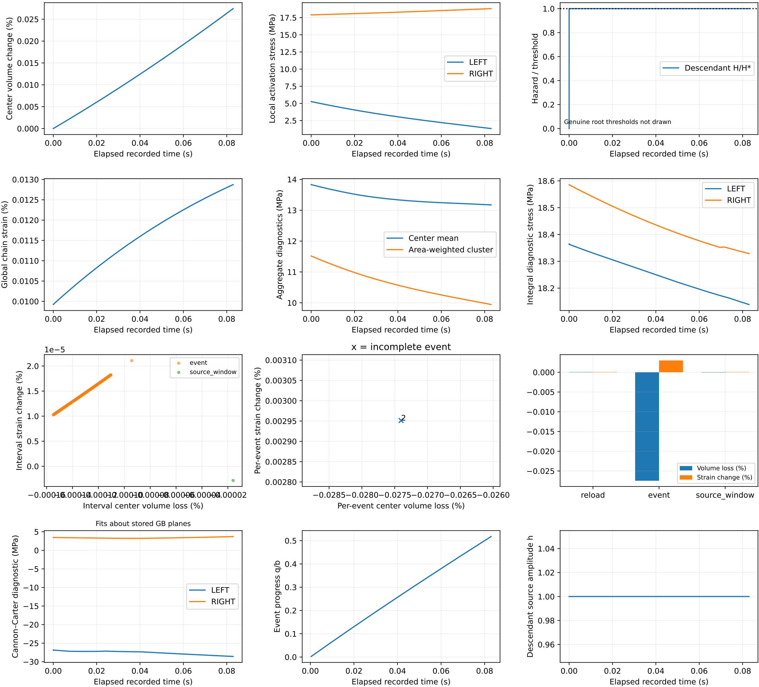
Conditional descendants after a forced root — not genuine root statistics
