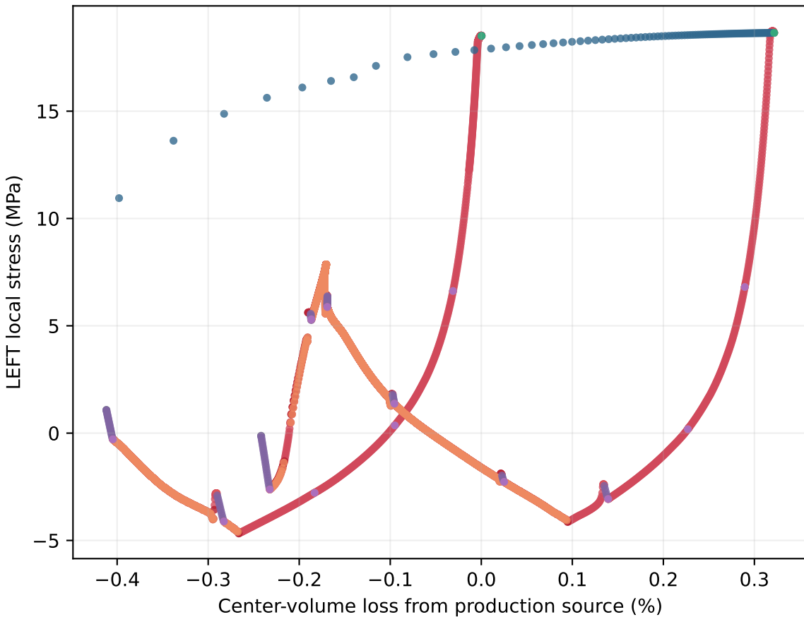
LEFT phase-resolved path
