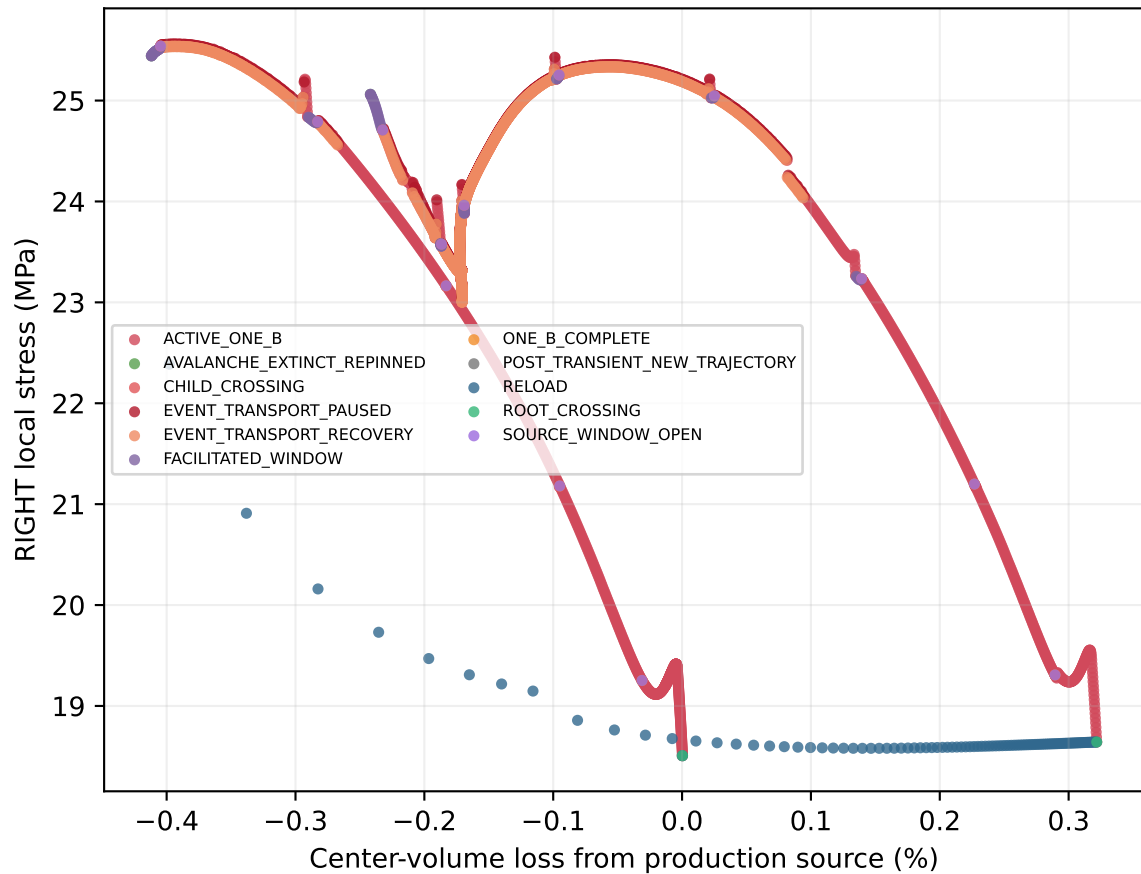
RIGHT phase-resolved path
