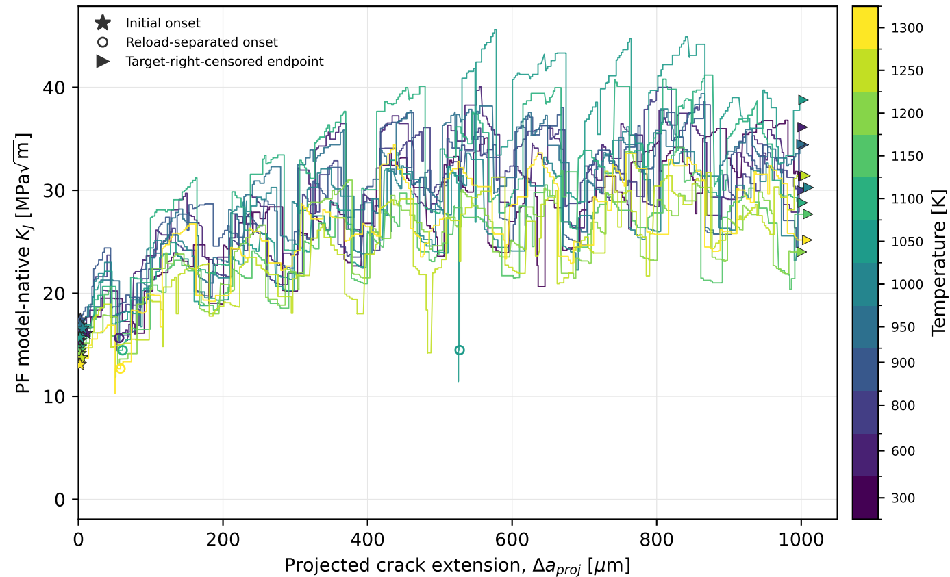
ceramic-like: theta=0 deg, rate=1x PF MODEL-NATIVE KJ TRAJECTORY — FULL RANGE
