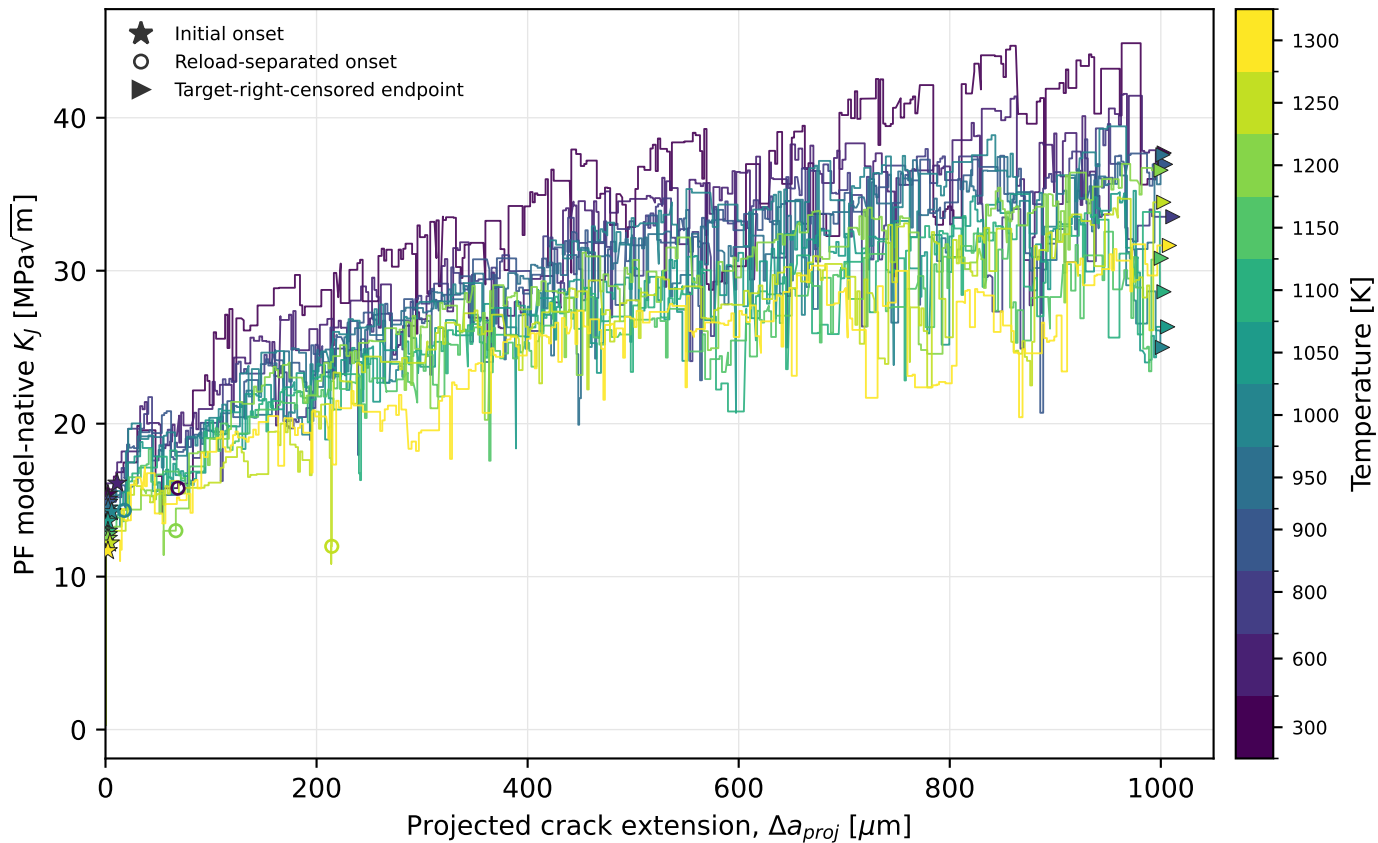
ceramic-like: theta=30 deg, rate=1x PF MODEL-NATIVE KJ TRAJECTORY — FULL RANGE
