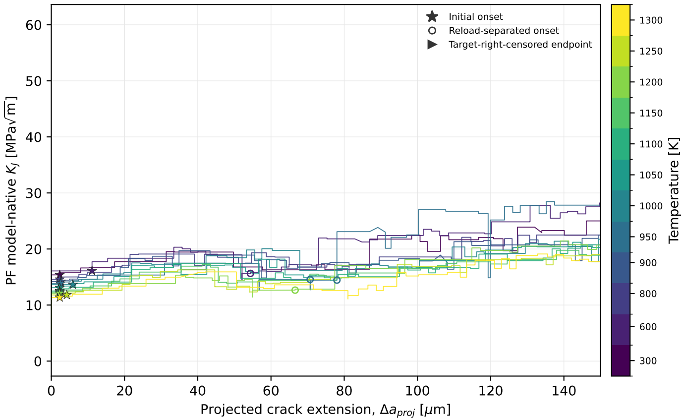
ceramic-like: theta=45 deg, rate=1x PF MODEL-NATIVE K J TRAJECTORY — EARLY RANGE
