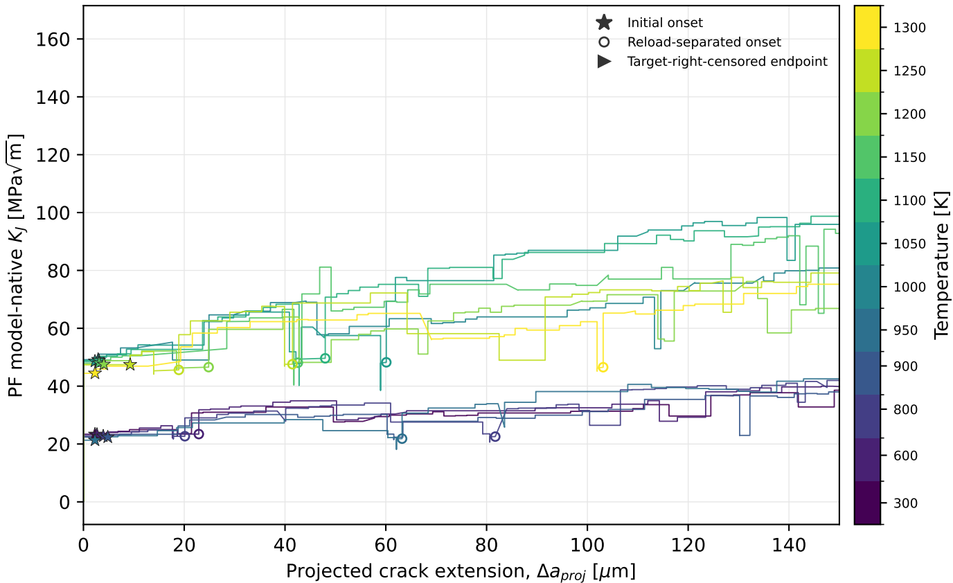
DBTT: theta=15 deg, rate=1x PF MODEL-NATIVE KJ TRAJECTORY — EARLY RANGE
