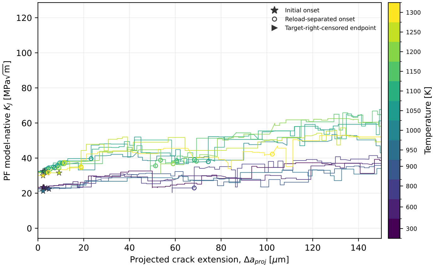
DBTT: theta=30 deg, rate=1x PF MODEL-NATIVE KJ TRAJECTORY — EARLY RANGE
