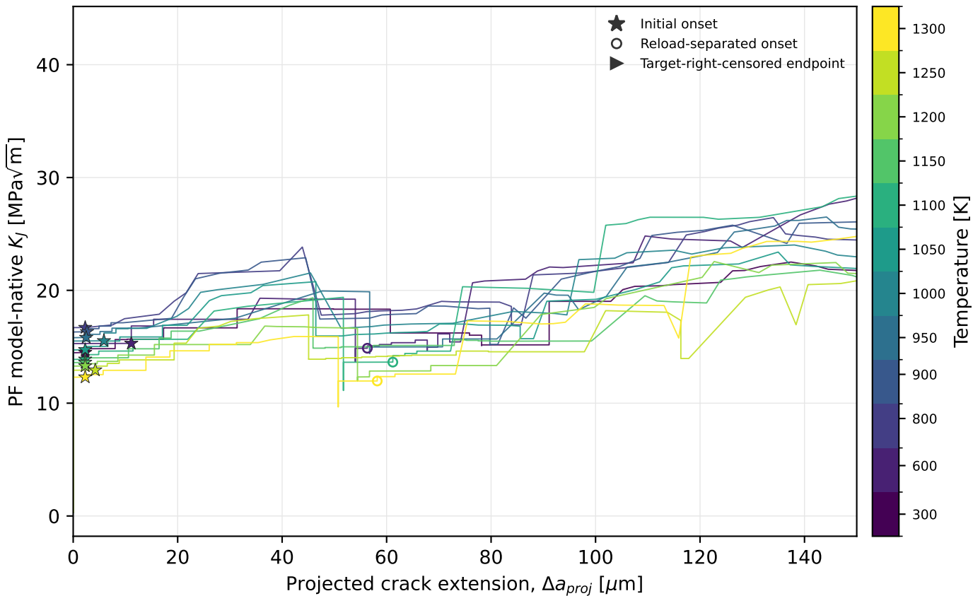
ceramic-like: theta=0 deg, rate0p01x PF MODEL-NATIVE KJ TRAJECTORY — EARLY RANGE
