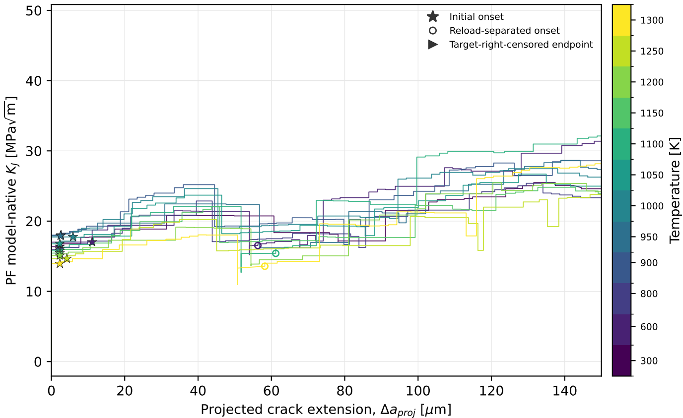
ceramic-like: theta=0 deg, rate100x PF MODEL-NATIVE KJ TRAJECTORY — EARLY RANGE
