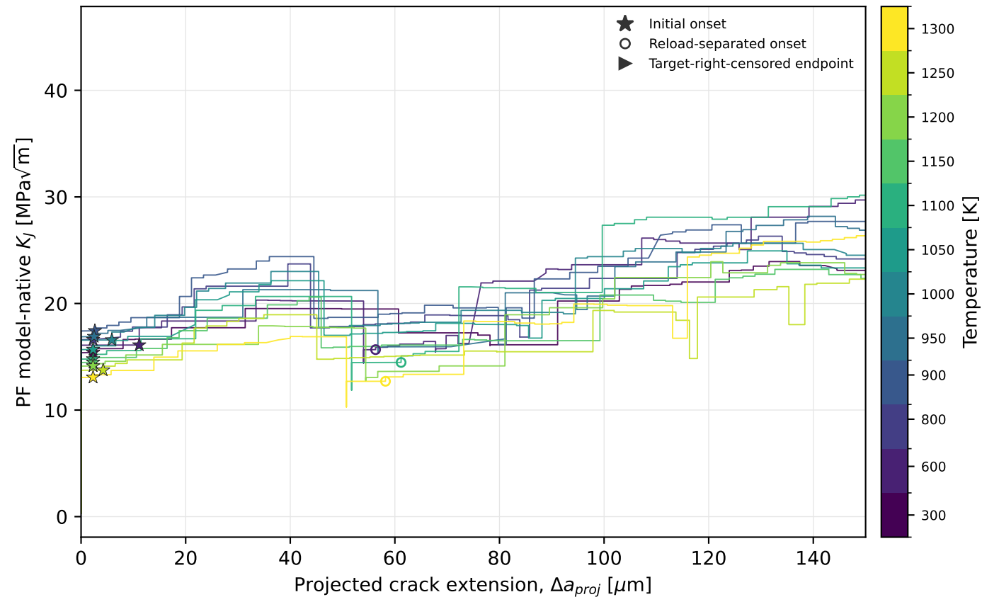
ceramic-like: theta=0 deg, rate1x PF MODEL-NATIVE K J TRAJECTORY — EARLY RANGE
